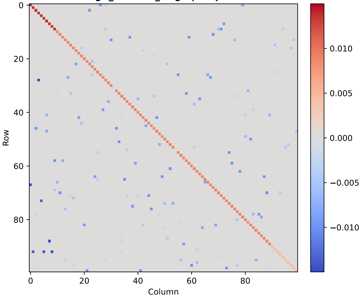
gd_random_large | step 7
